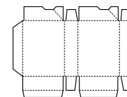
Lock - bottom
